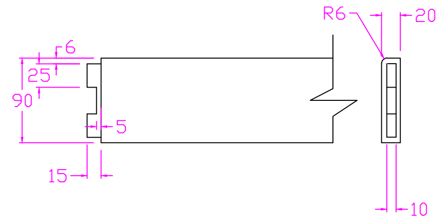
SIDE RAIL - TENONS TRAVERSE LATERALE - TENONS
