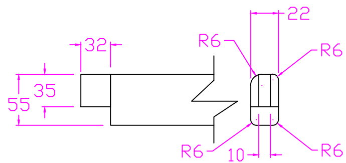
UPPER SIDE RAIL - TENON TRAVERSE LATERALE SUPERIEURE - TENONS
