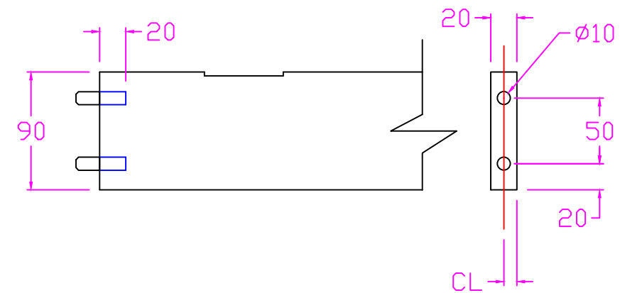
BACK RAIL - DOWELS TRAVERSE ARRIERE - GOUJONS
